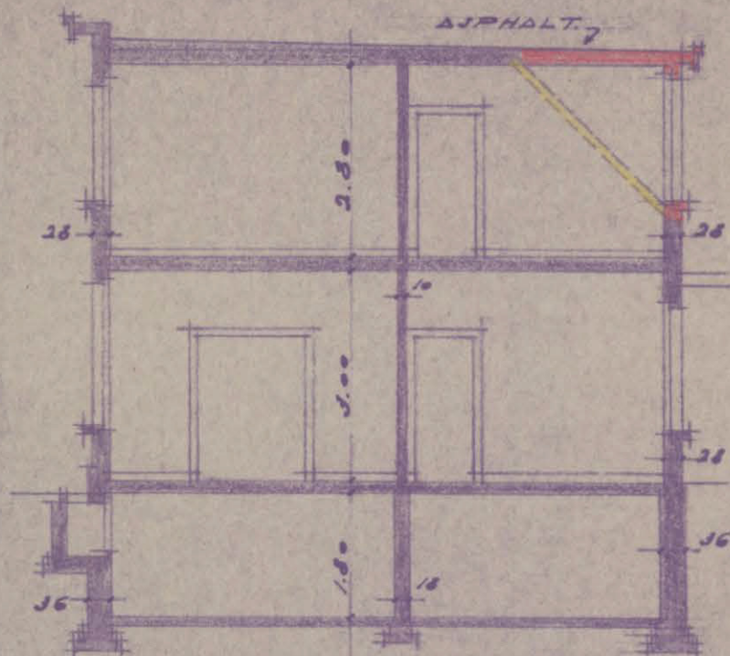
DOORSNED: A.B.
