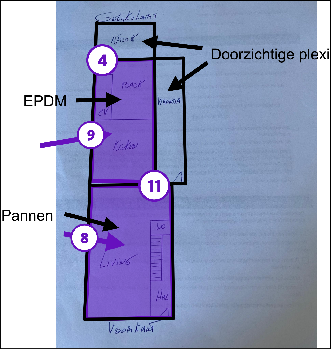
Legende van plan 1.6: Dakenplan
