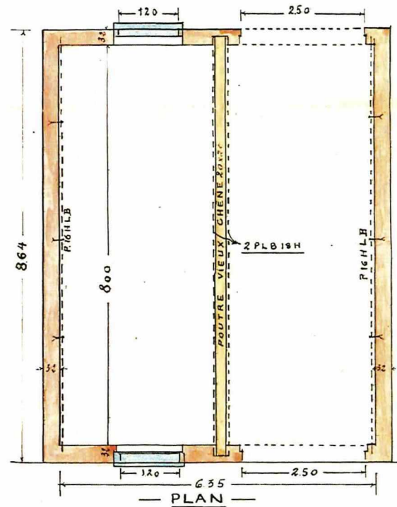
PLAN
