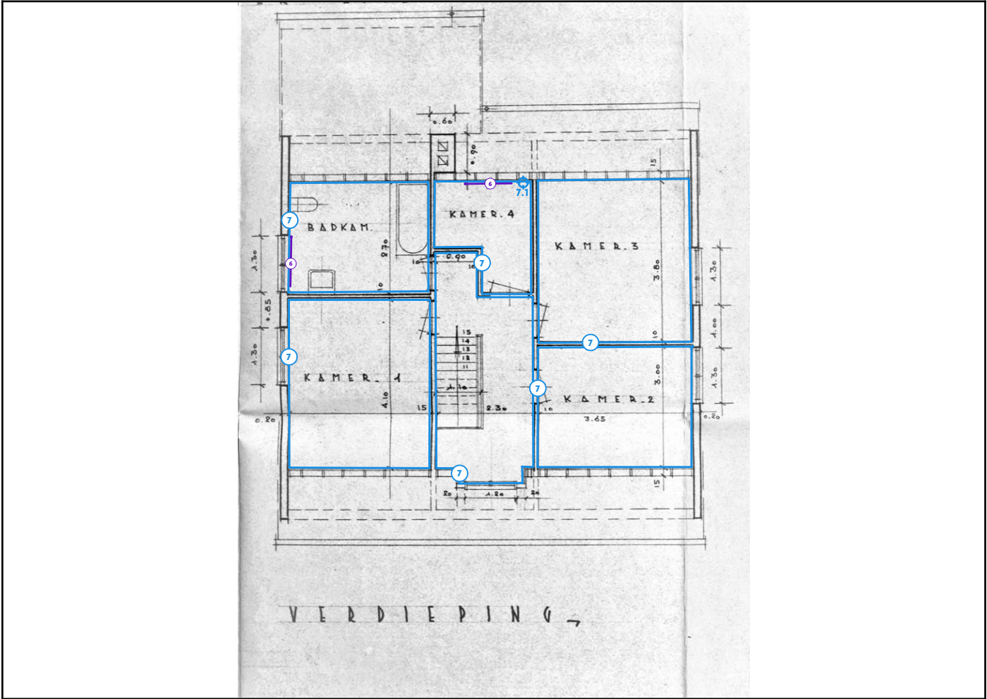
Legende van plan 1.5: Verdieping +1
