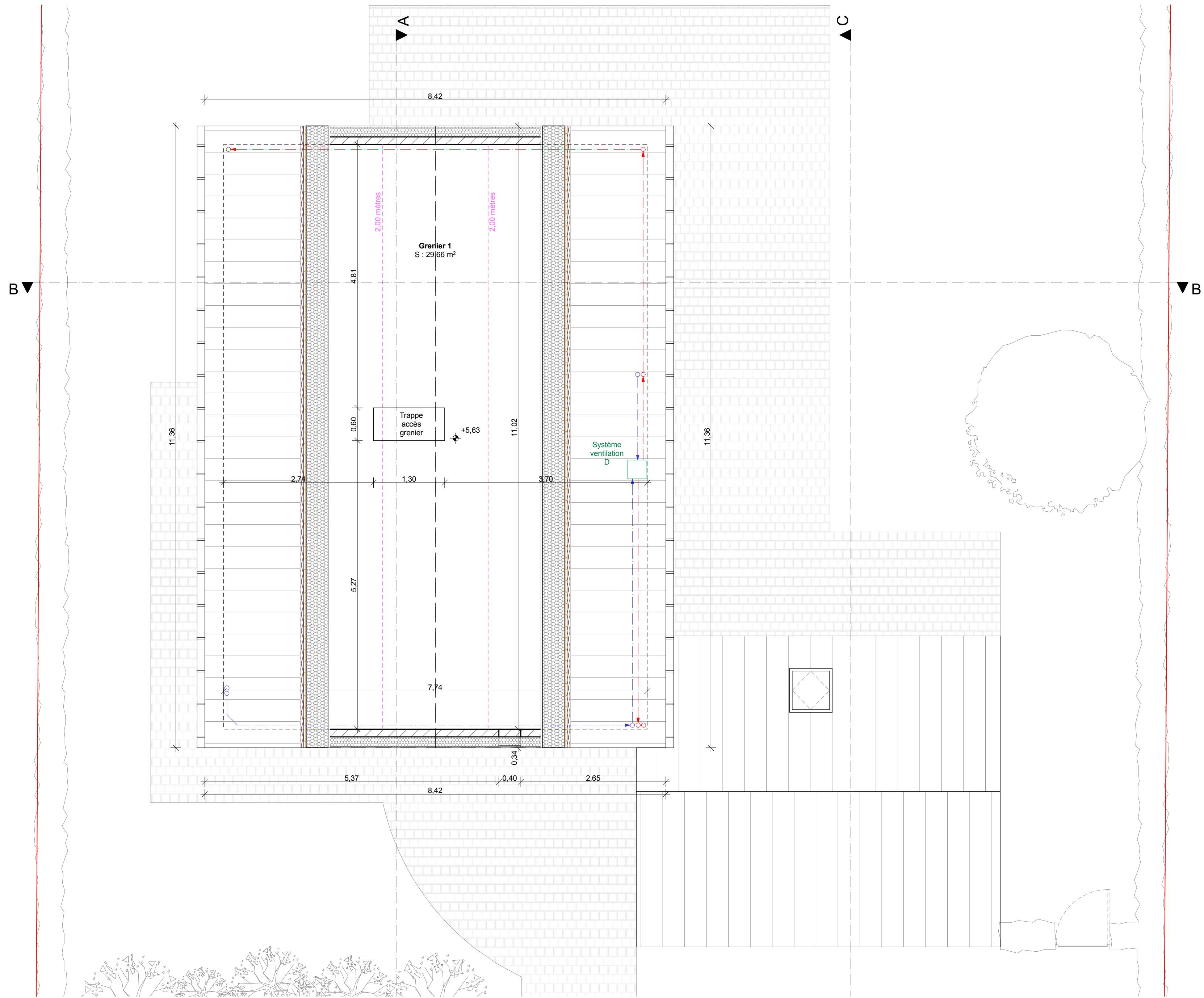
Combles
