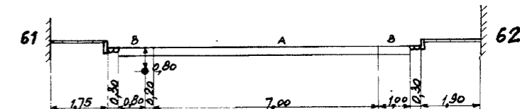
DOORSNEDE 31-31
